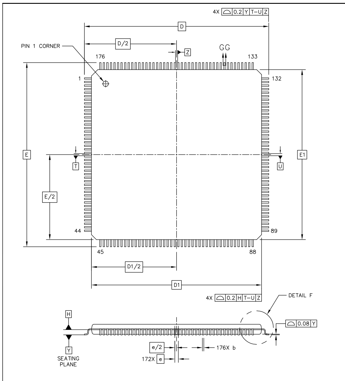
Figure 33. 176 LQFP package mechanical drawing (Part 1 of 3)
