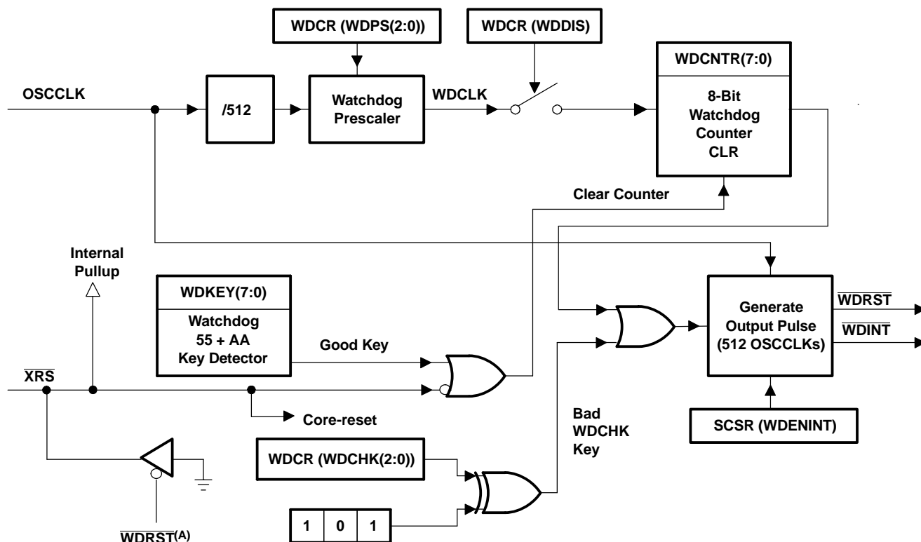
Figure 3-13. Watchdog Module
