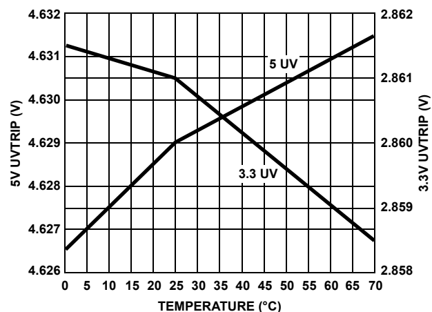
FIGURE 5. UV TRIP vs TEMPERATURE (HIP1011D only)
