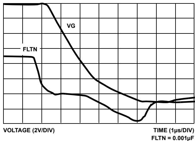
FIGURE 21. FLTN TO 35VG DELAY
