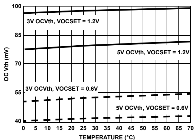
FIGURE 7. OC V_{th} vs TEMPERATURE
