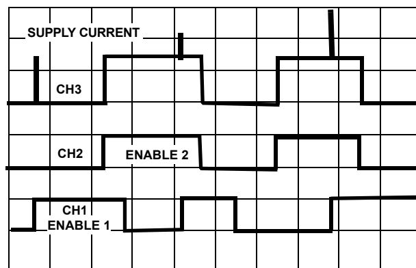
FIGURE 19. HIP1011DEVAL1 3.3V SUPPLY CURRENT AS CONTROLLER 1 TURNS ON INTO SHORTED LOAD CARD
