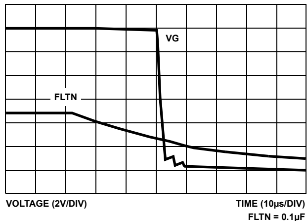
FIGURE 23. FLTN TO 35VG DELAY
