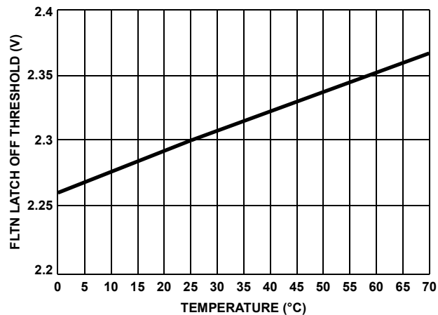
FIGURE 13. FLTN LATCH-OFF THRESHOLD VOLTAGE vs TEMPERATURE
