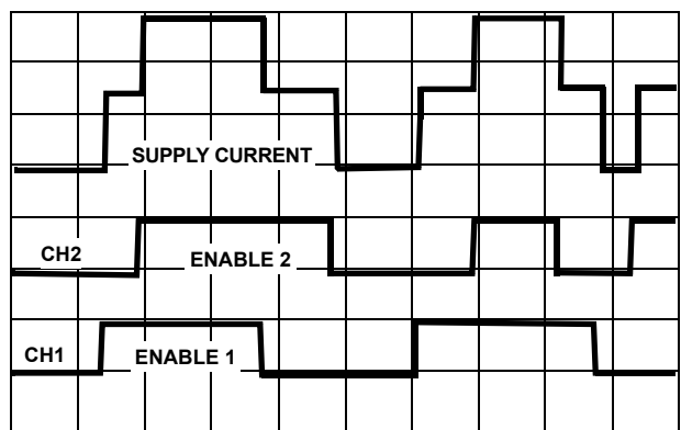
FIGURE 18. HIP1011DEVAL1 3.3V SUPPLY CURRENT AS EACH SLOT CONTROLLER TURNS ON INTO LOAD CARD
