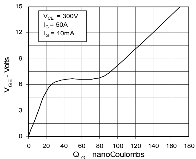
Fig. 14. Gate Charge
