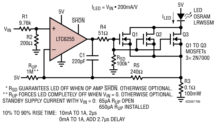
Figure 6. LTC6255 Applied as a LED Current Driver with 2μs Rise Time
