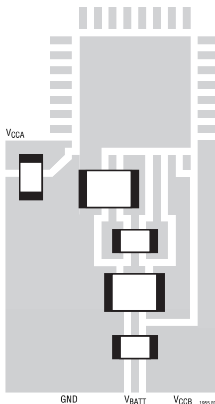
Figure 3. Optimum Single-Layer PCB Layout
