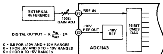
Figure 5. External Reference
