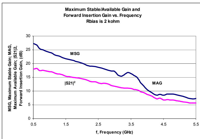
Figure 2. Maximum Stable/Available Gain and Forward Insertion Gain vs. Frequency ( R_{bias} = 2\text{ k}\Omega )
