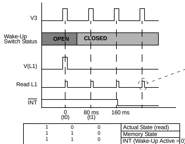
Figure 11. Cyclic Sense Timing
