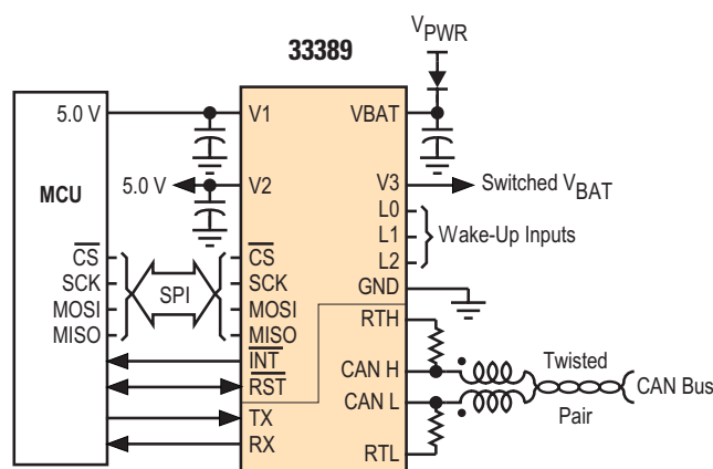
Figure 1. 33389 Simplified Application Diagram
