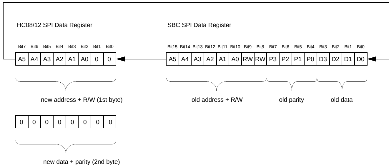
Figure 19. Microcontroller SPI Reading Data - Sequence A
