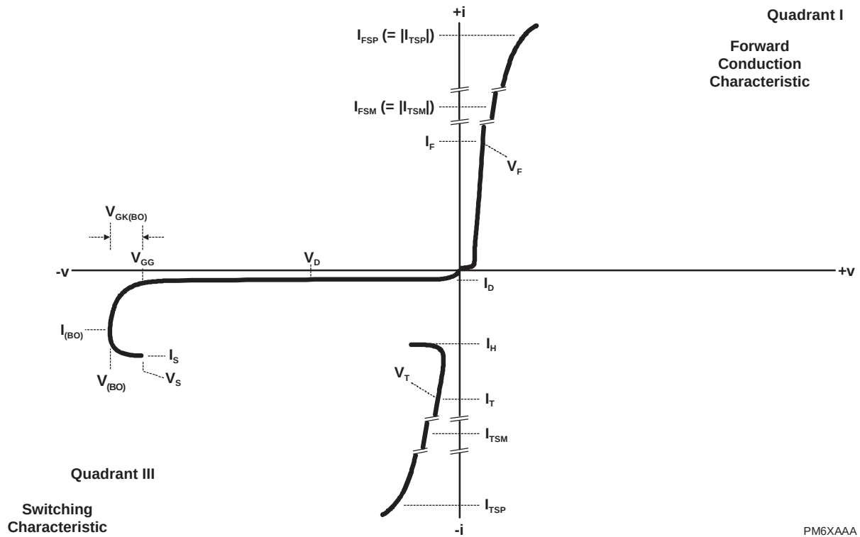
Figure 1. Voltage-Current Characteristic
