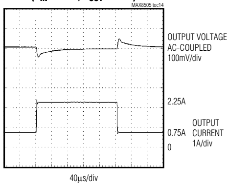
TRANSIENT RESPONSE ( V_{IN} = 3.3V , V_{OUT} = 1.2V )
