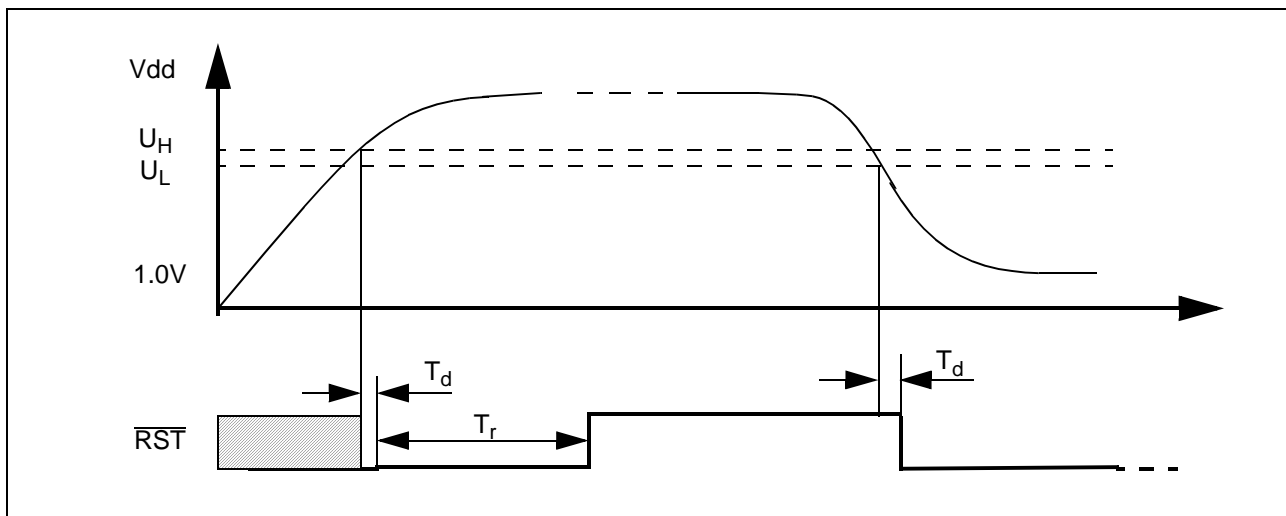
Figure 21 UVD Timing Characteristics
