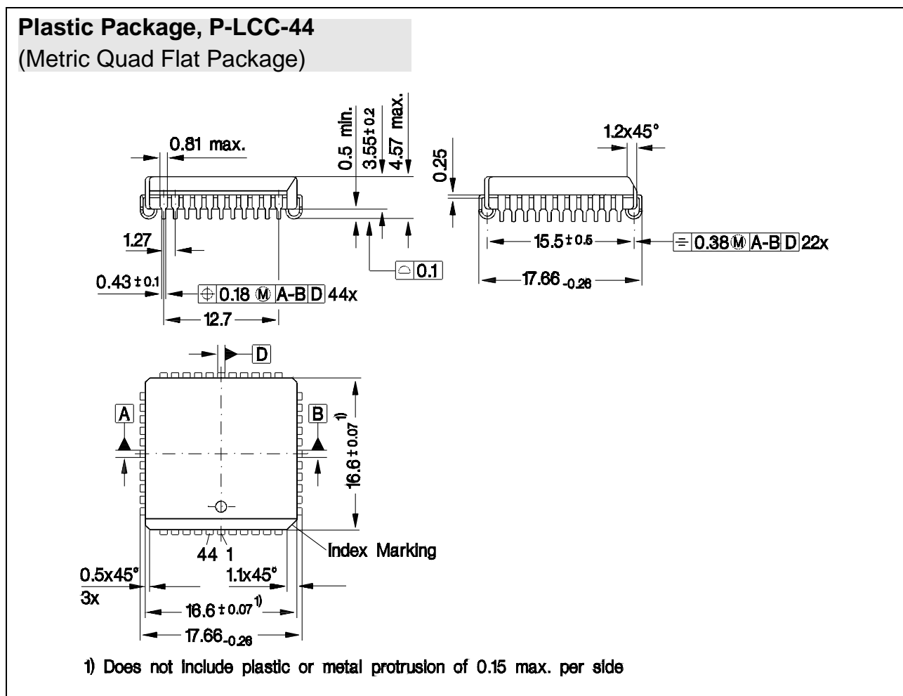
Figure 24 Package Outline for P-LCC-44
