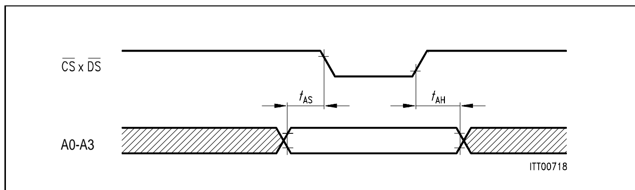
Figure 20 Motorola Non-Multiplexed Address Timing
