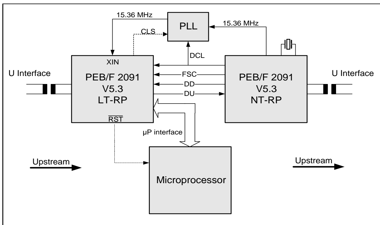
Figure 2 Architecture of Repeater Application
