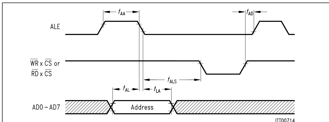
Figure 16 Siemens/Intel Multiplexed Address Timing
