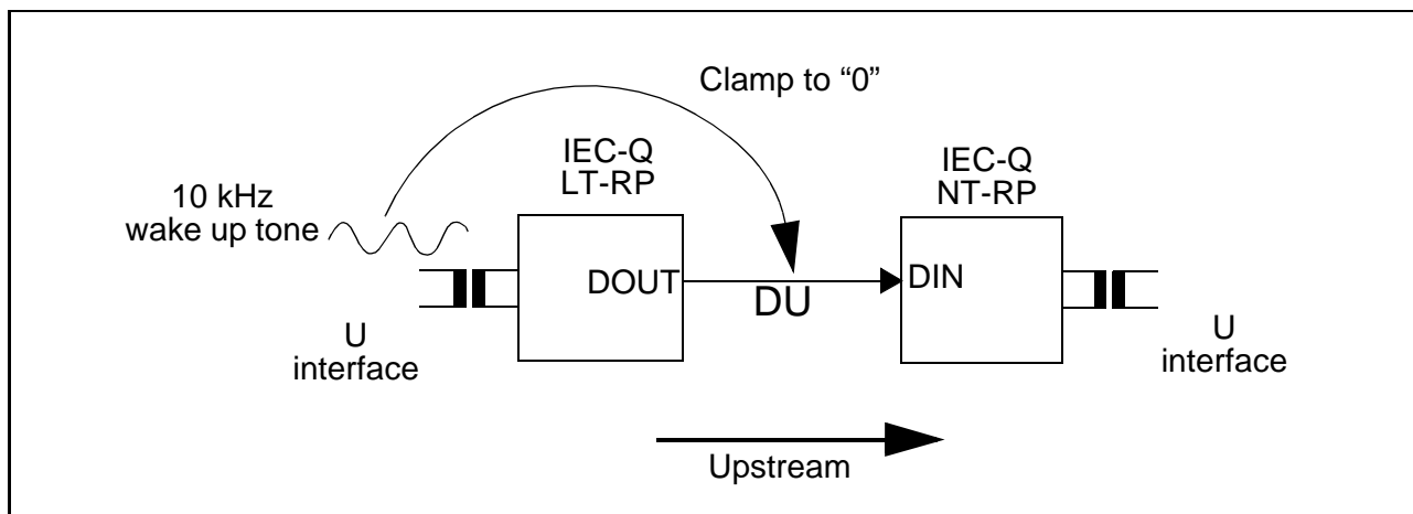
Figure 6 Wake Up Indication in Repeater Power Down
