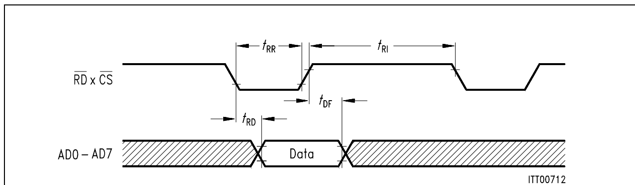
Figure 14 Siemens/Intel Read Cycle
