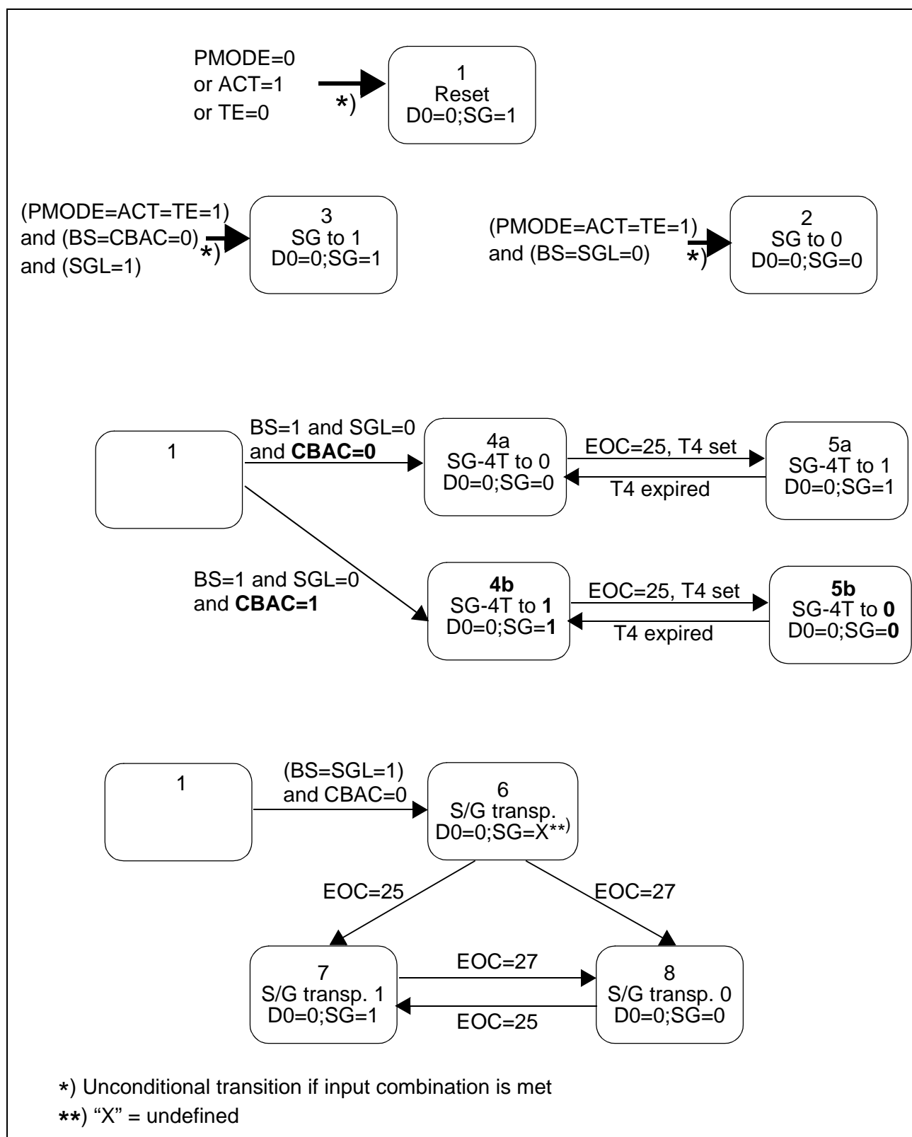
Figure 9 State Machine for S/G Bit Control (part 1)
