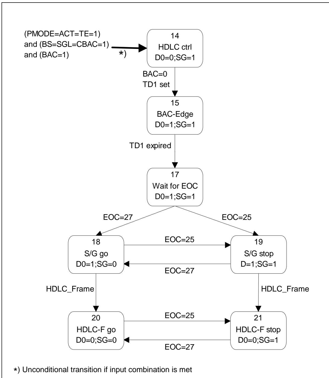
Figure 11 State Machine for S/G Bit Control (Part 3)
