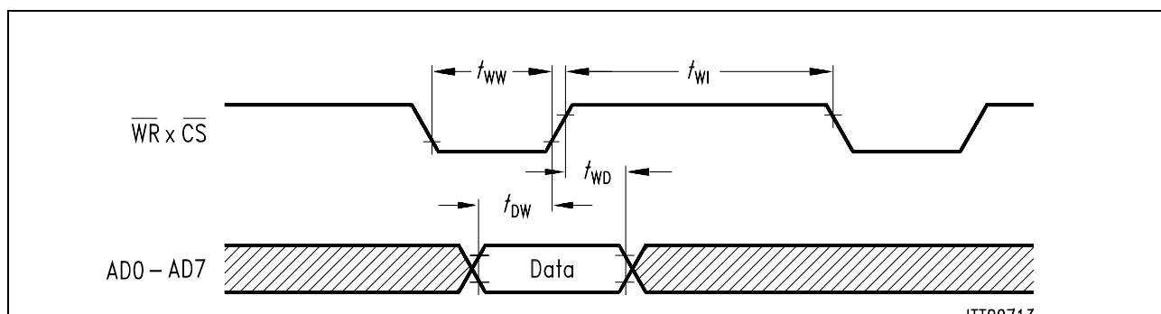
Figure 15 Siemens/Intel Write Cycle
