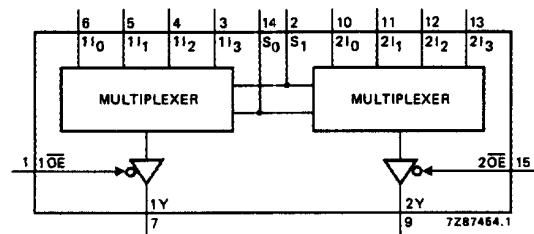
Fig.4 Functional diagram.
