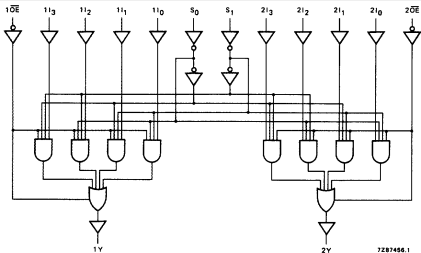
Fig.5 Logic diagram.
