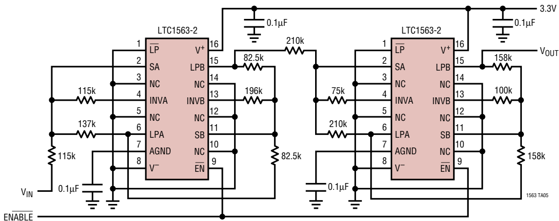
Single 3.3V, 2mA Supply current, 20kHz 8th Order Butterworth Lowpass Filter
