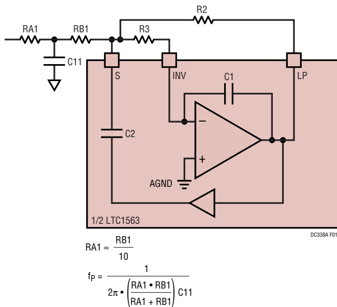
Figure 2. Input TEE Network
