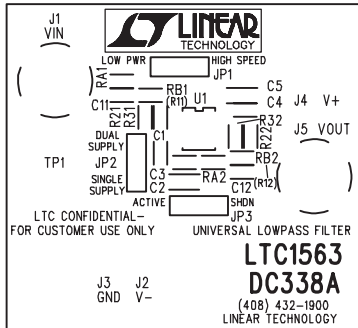
Silkscreen Top
