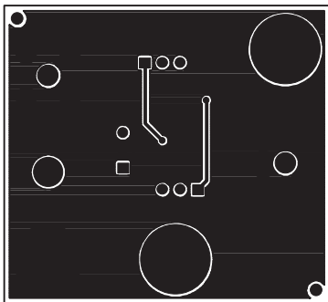
Solder Side
