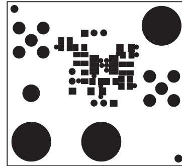
Solder Mask Top
