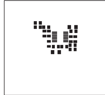
Paste Mask Top
