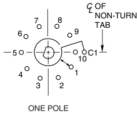
ONE POLE
