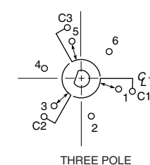
THREE POLE
