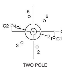
TWO POLE
