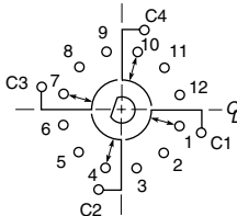
FOUR POLE
