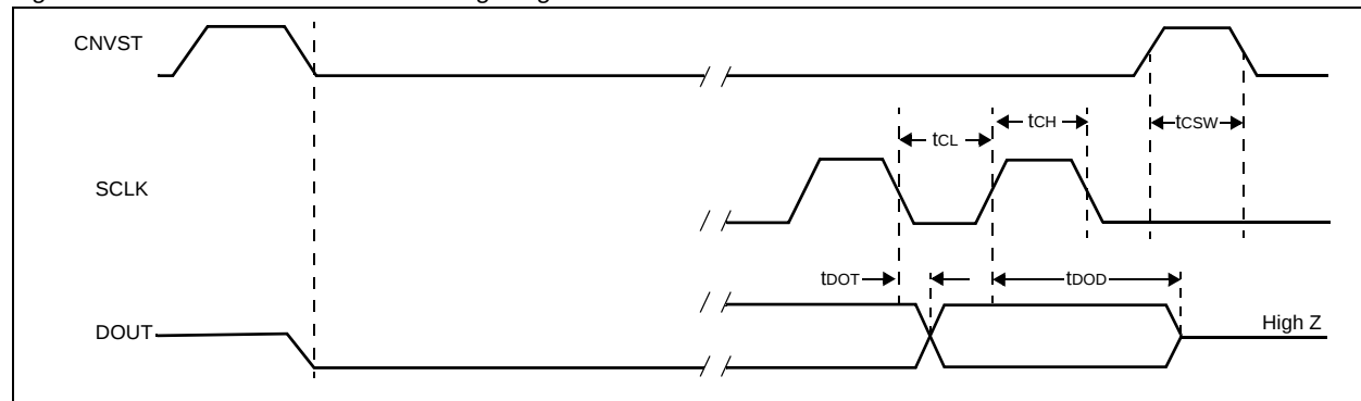
Figure 4. Detailed Serial Interface Timing Diagram
