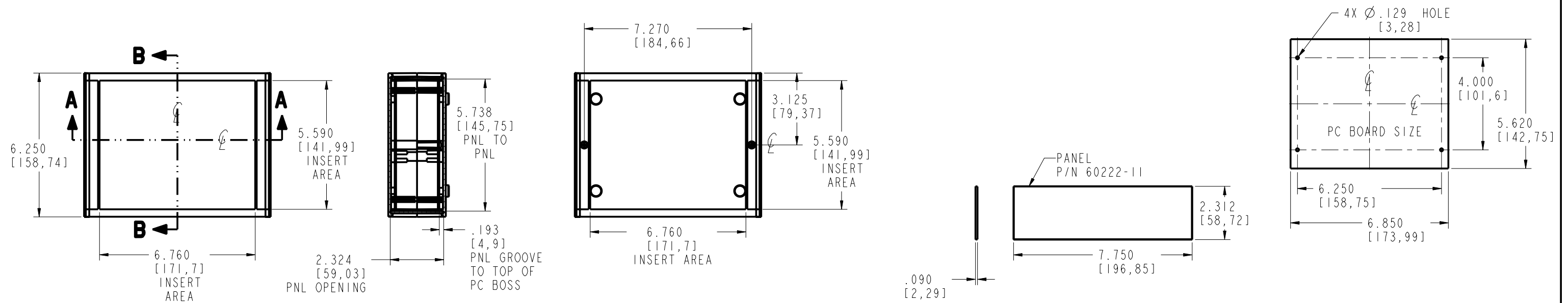
SECTION B-B
