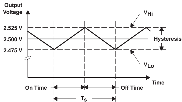
Figure 1–2. Simplified Hysteretic Controlled Output Voltage Waveform
