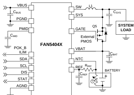
Figure 1. Typical Application
