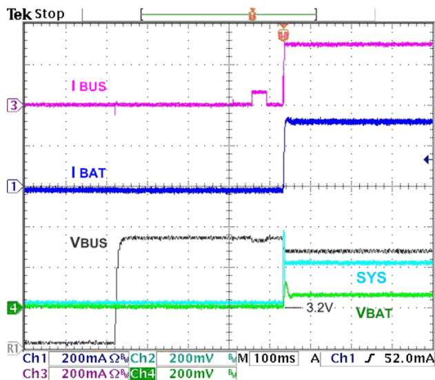
Figure 13. Charger Startup at V_{\text{BUS}} Plug-In Using 300 mA Current Limited Source, 500 mA I_{\text{BUSLIM}} , 3.2 V V_{\text{BAT}} , 50 \Omega \text{SYS} Load
