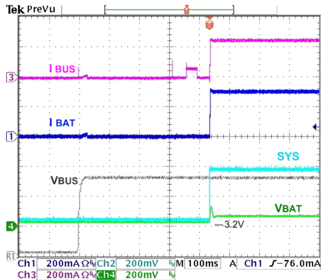
Figure 12. Charger Startup at V_{\text{BUS}} Plug-In, 500 mA I_{\text{BUSLIM}} , 3.2 V V_{\text{BAT}} , 100 \Omega \text{SYS} Load
