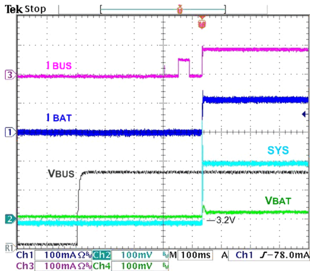
Figure 11. Charger Startup at V_{\text{BUS}} Plug-In, 100 mA I_{\text{BUSLIM}} , 3.2 V V_{\text{BAT}} , 100 \Omega \text{SYS} Load
