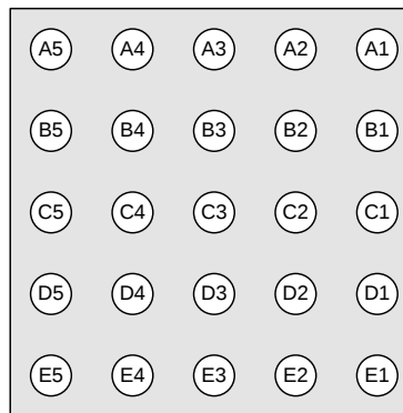
Figure 4. Bottom View
