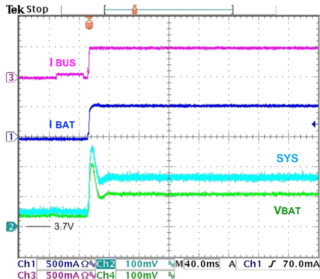
Figure 14. Charger Startup with HZ Bit Reset, 500 mA I_{\text{BUSLIM}} , 950 mA I_{\text{CHARGE}} , 50 \Omega \text{SYS} Load
