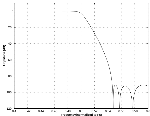
Figure 10. Single-Speed (fast) Transition Band
