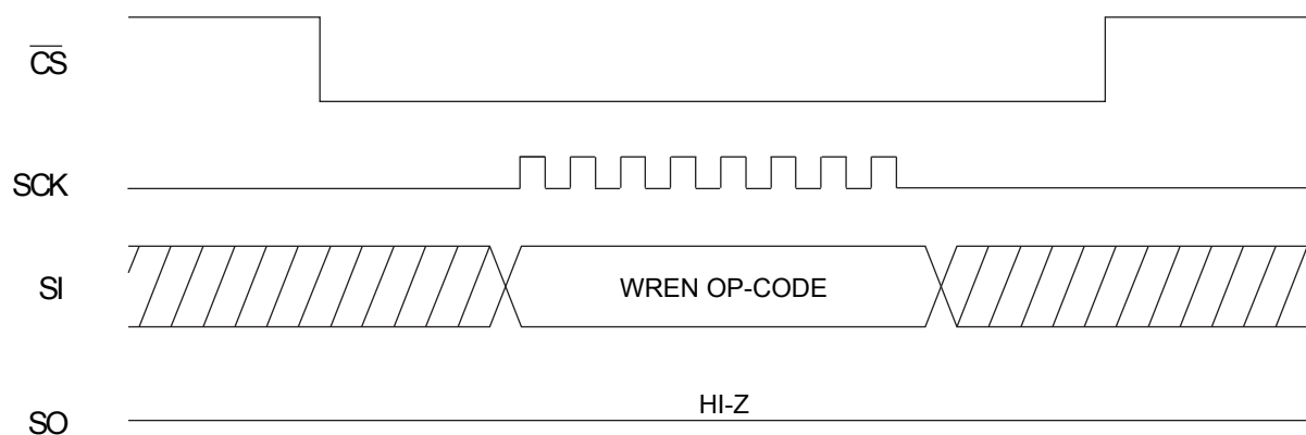
Figure K-1. SPI Write Enable (WREN) Timing
