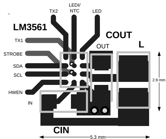
Figure 2. Example Layout
