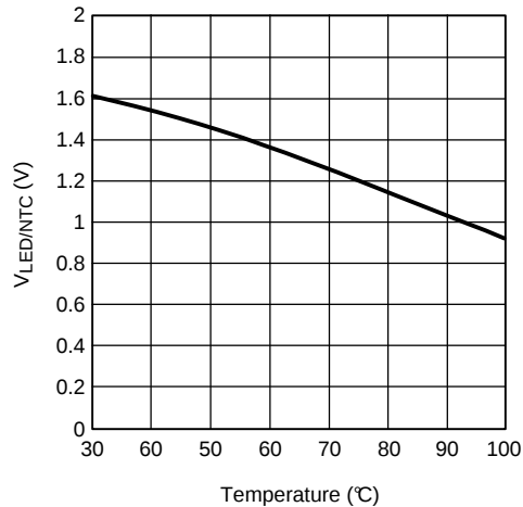
Figure 39. Thermistor Resistive Divider Response vs Temperature VLEDI/NTC vs Temp ( V_{BIAS} = 1.8V , THERMISTOR = 10k\Omega at +25^{\circ}C , \beta = 3380 , R_{BIAS} = 972\Omega )
