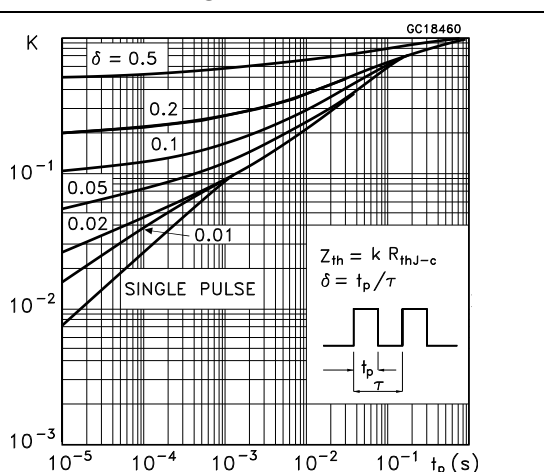
Figure 5. Thermal impedance for TO-247 and TO-247LL
