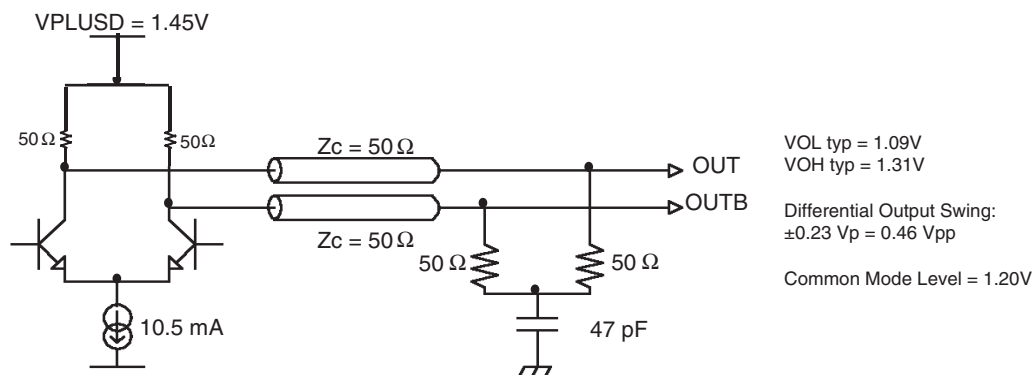
Figure 8-9. 50 \Omega Terminated Differential Outputs
