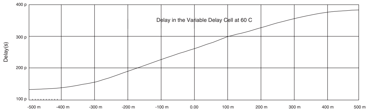
Figure 8-14. Typical Tuning Range is \pm 120 ps for Applied Control Voltage Varying Between -0.5 V to 0.5 V on SDA Pin
