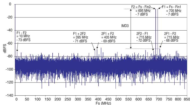
Figure 4-13. Dual Tone Signal Spectrum at F_s = 1.7 Gps, F_{in1} = 995 MHz, F_{in2} = 1005 MHz (–7 dBFS), IMD3 = 68 dBFS.
