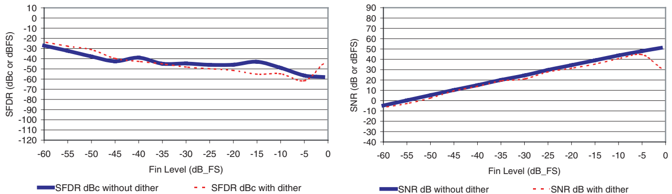
Figure 4-12. SFDR and SNR (dBc and dBFS) with and without Added Dither (–17 dBm DC to 5 MHz out of Band Dither) vs. Analog Input Power at F_s = 1.7 Gps, F_{in} = 710 MHz
