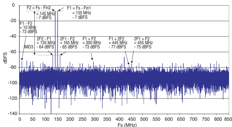
Figure 4-15. Dual Tone Signal Spectrum at F_s = 1.7 Gsps, F_{in1} = 1945 MHz, F_{in2} = 1955 MHz ( -7 dBFS), IMD3 = 59 dBFS
