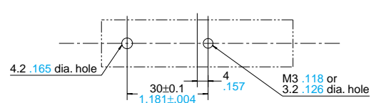
Mounting hole dimensions
