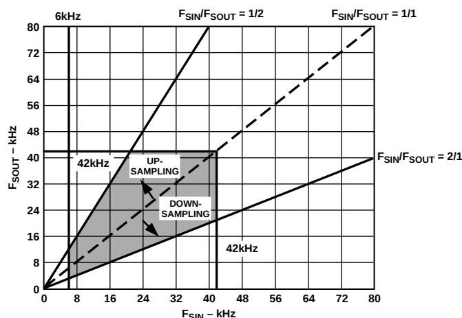
Figure 12. Allowable Input and Output Sample Frequencies F_{\text{CRYSTAL}} = 12 \text{ MHz} Case
