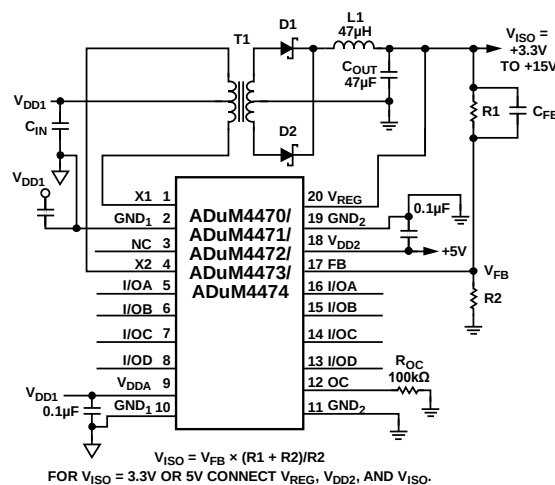
Figure 48. Single Power Supply
