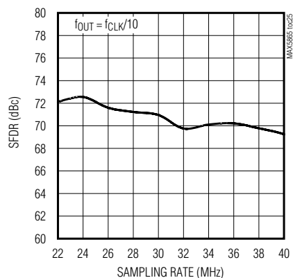
DAC SPURIOUS-FREE DYNAMIC RANGE vs. SAMPLING RATE
