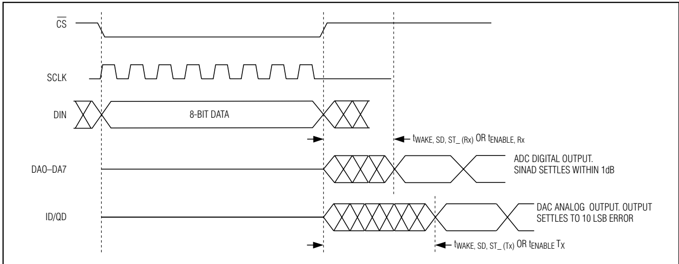
Figure 6. MAX5865 Mode Recovery Timing Diagram
