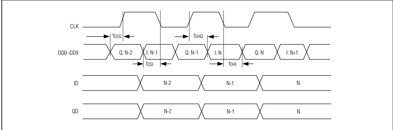
Figure 4. DAC System Timing Diagram
