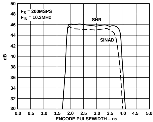
Figure 15. SNR vs. Clock Pulsewidth, ( t_{PWH} ): f_S = 200 MSPS
