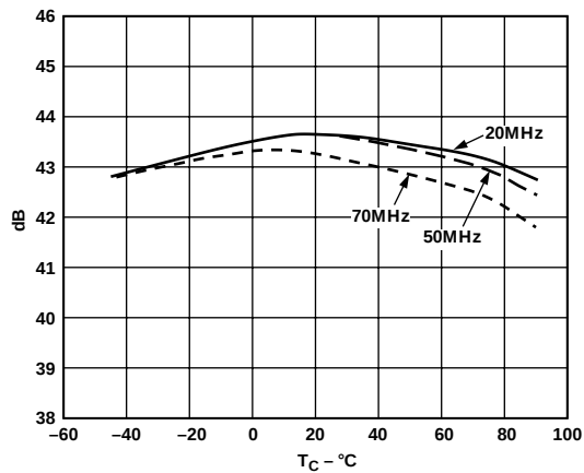
Figure 16. SINAD vs. Temperature: f_S = 135 MSPS
