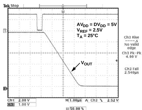
Figure 11. Slew Rate with Boost Off
