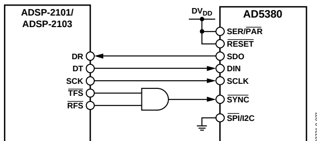
Figure 38. AD5380-to-ADSP-2101/ADSP-2103 Interface
