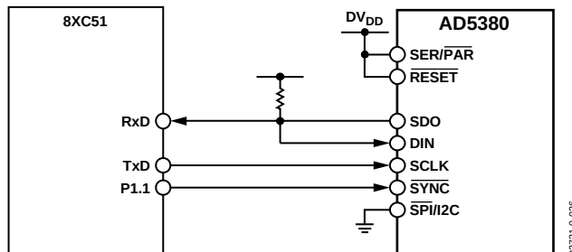
Figure 37. AD5380-to-8051 Interface
