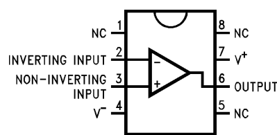
8-Pin DIP/SO
