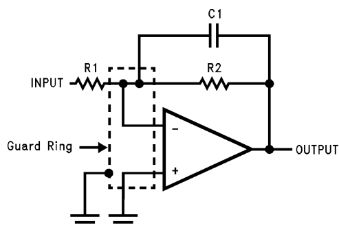
FIGURE 5. Inverting Amplifier Guard Ring Connections
