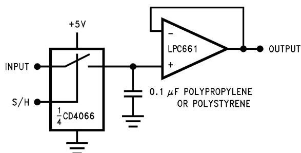
Low-Leakage Sample-and-Hold
