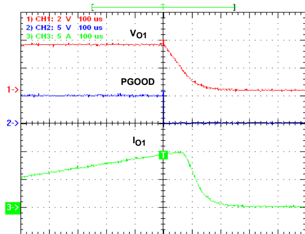
FIGURE 20. OVERCURRENT PROTECTION, V_{IN} = 12V , V_O = 3.3V
