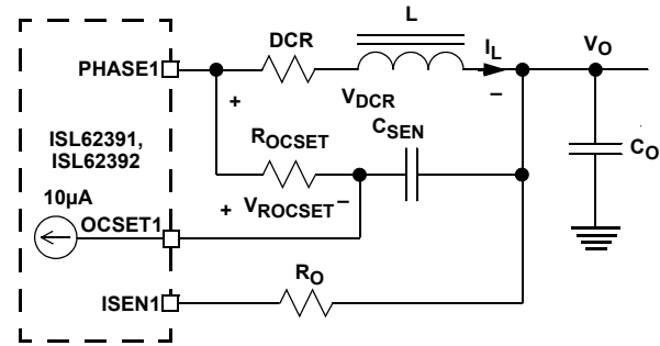
FIGURE 26. OVERCURRENT-SET CIRCUIT
