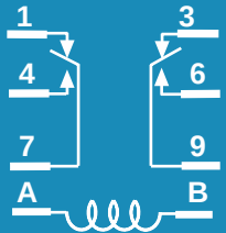
DPDT
