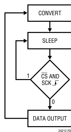
Figure 2. LTC2421/LTC2422 State Transition Diagram
