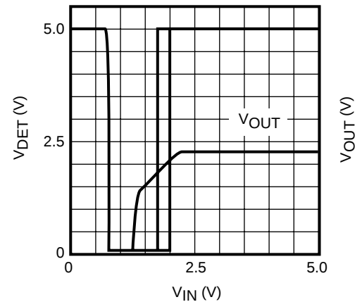
LOW VOLTAGE DETECTOR vs. INPUT VOLTAGE
