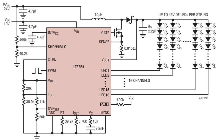
92% Efficient, 36W Backlight LED Driver
