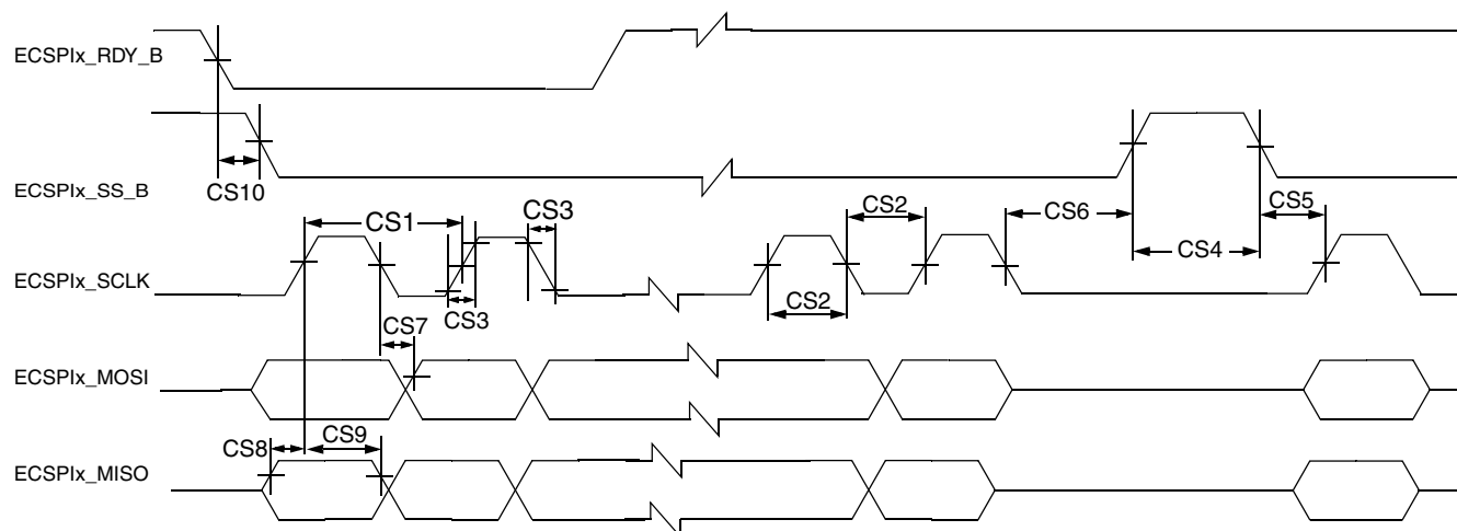
Figure 39. ECSPi Master Mode Timing Diagram
