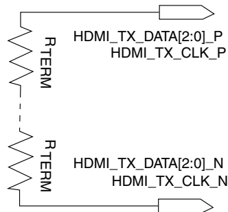
Figure 56. Source Termination
