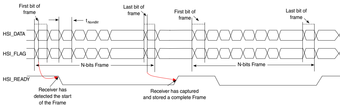
Figure 77. Synchronized Data Flow READY Signal Timing (Frame and Stream Transmission)
