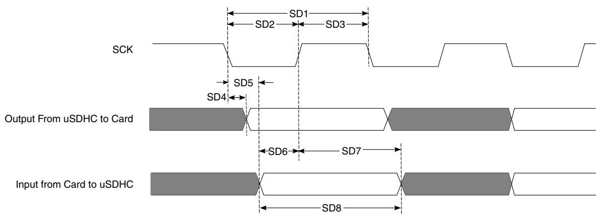
Figure 45. SDR50/SDR104 Timing
