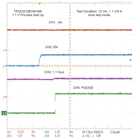
Figure 7-9. Output 1.1-V Prebias Turn-On
