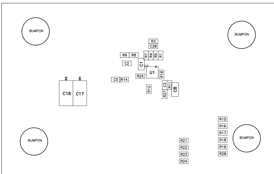
Figure 8-2. TPS53219EVM-690 Bottom Assembly Drawing, Bottom View
