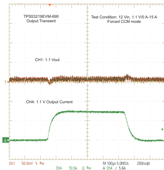
Figure 7-3. Output Load Transient
