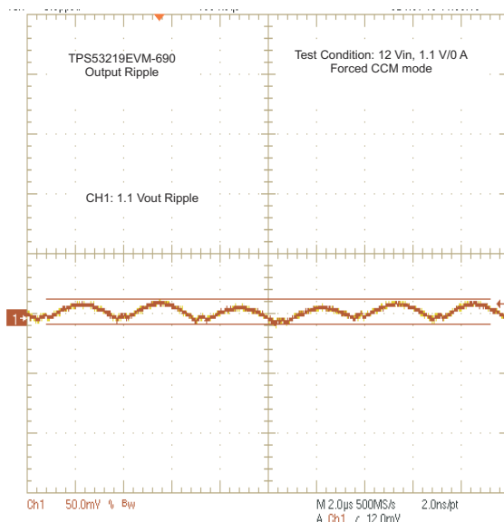
Figure 7-5. Output Ripple
