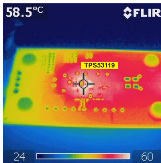
Figure 7-12. Bottom Board at 12 V IN , 1.1 V/25 A
