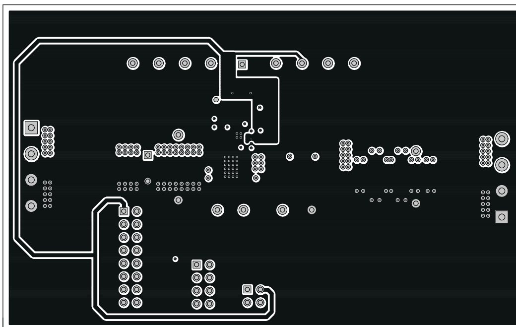
Figure 8-4. TPS53219EVM-690 Layer-2 Copper, Top View
