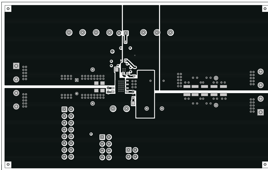
Figure 8-3. TPS53219EVM-690 Top Copper, Top View
