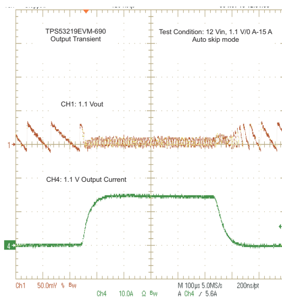
Figure 7-4. Output Load Transient
