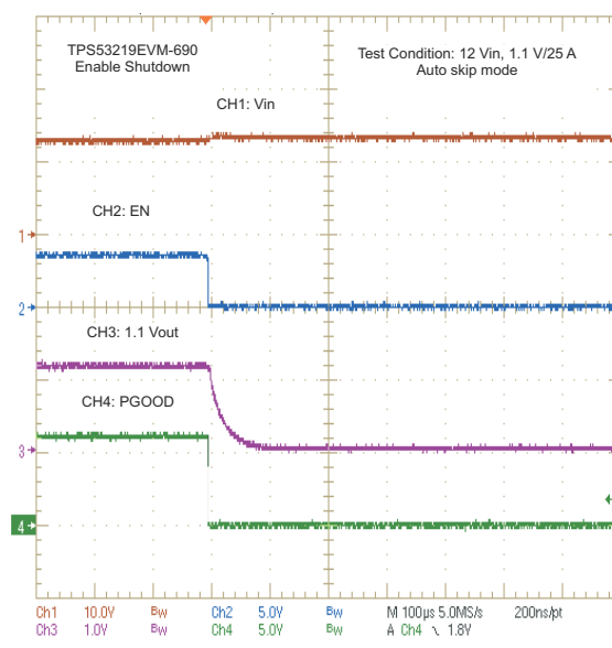
Figure 7-8. Enable Turn-Off
