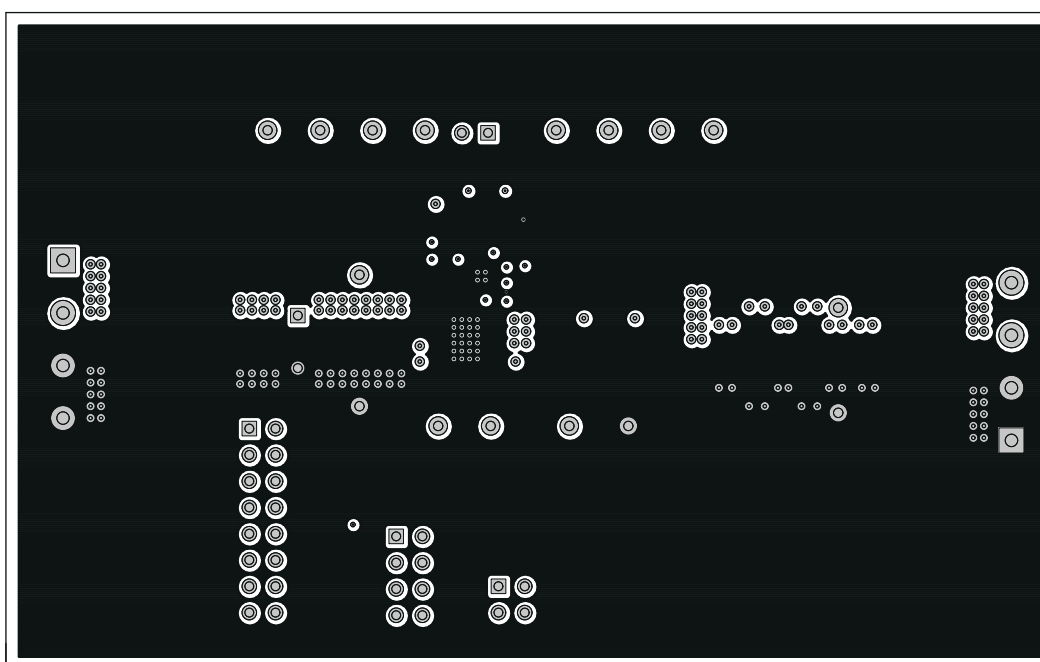
Figure 8-6. TPS53219EVM-690 Layer-4 Copper, Top View
