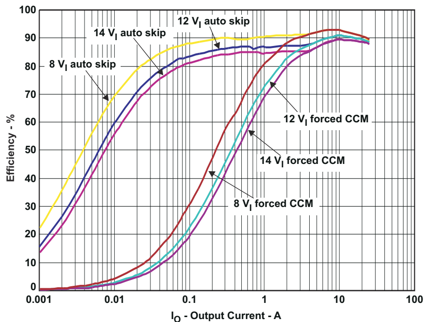
Figure 7-1. Efficiency
