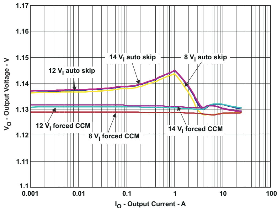
Figure 7-2. Load Regulation
