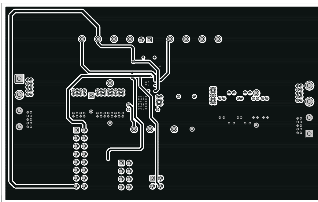
Figure 8-5. TPS53219EVM-690 Layer-3 Copper, Top View
