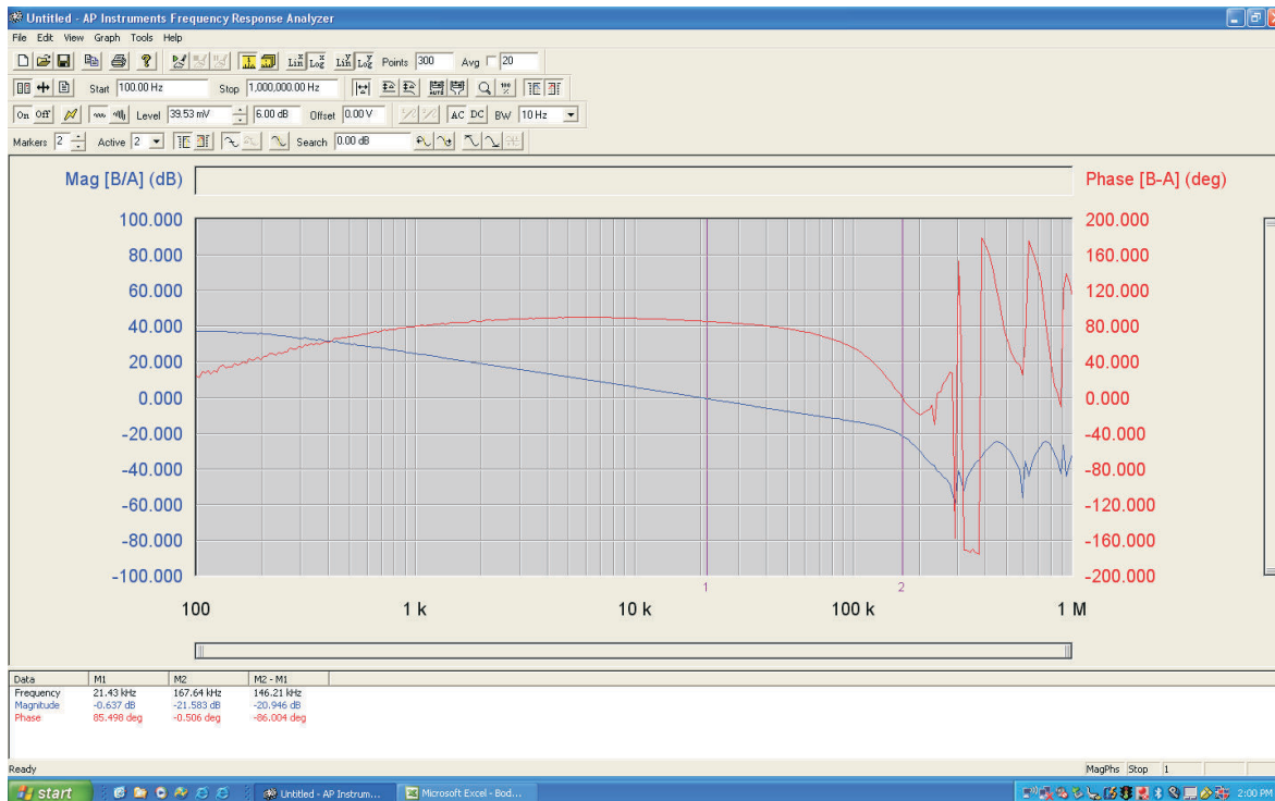
Figure 7-10. Bode Plot at 12 V IN , 1.1 V/25 A
