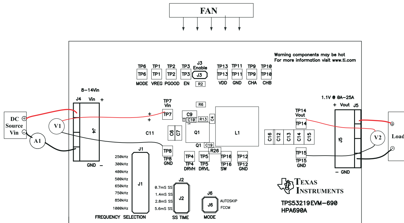
Figure 4-2. TPS53219EVM-690 Recommended Test Setup
