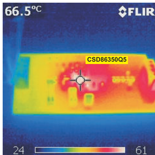
Figure 7-11. Top Board at 12 V IN , 1.1 V/25 A
