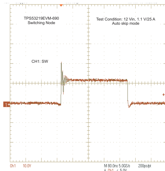
Figure 7-6. Switching Node
