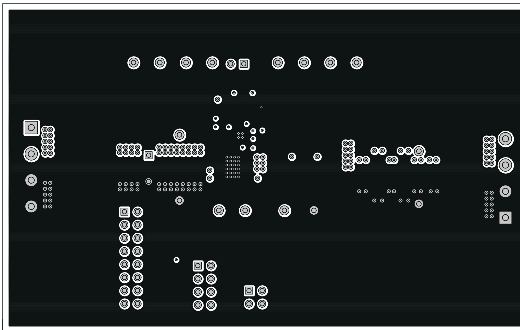
Figure 8-7. TPS53219EVM-690 Layer-5 Copper, Top View
