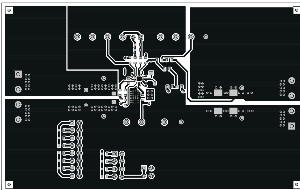
Figure 8-8. TPS53219EVM-690 Bottom Layer Copper, Top View
