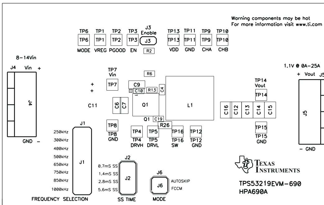
Figure 8-1. TPS53219EVM-690 Top Layer Assembly Drawing, Top View
