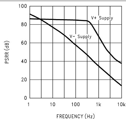
Figure 5-8. Power Supply Rejection Ratio vs Frequency
