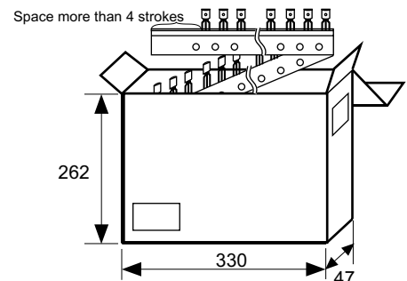
No. YZ003-C-Z-SD-2.0
