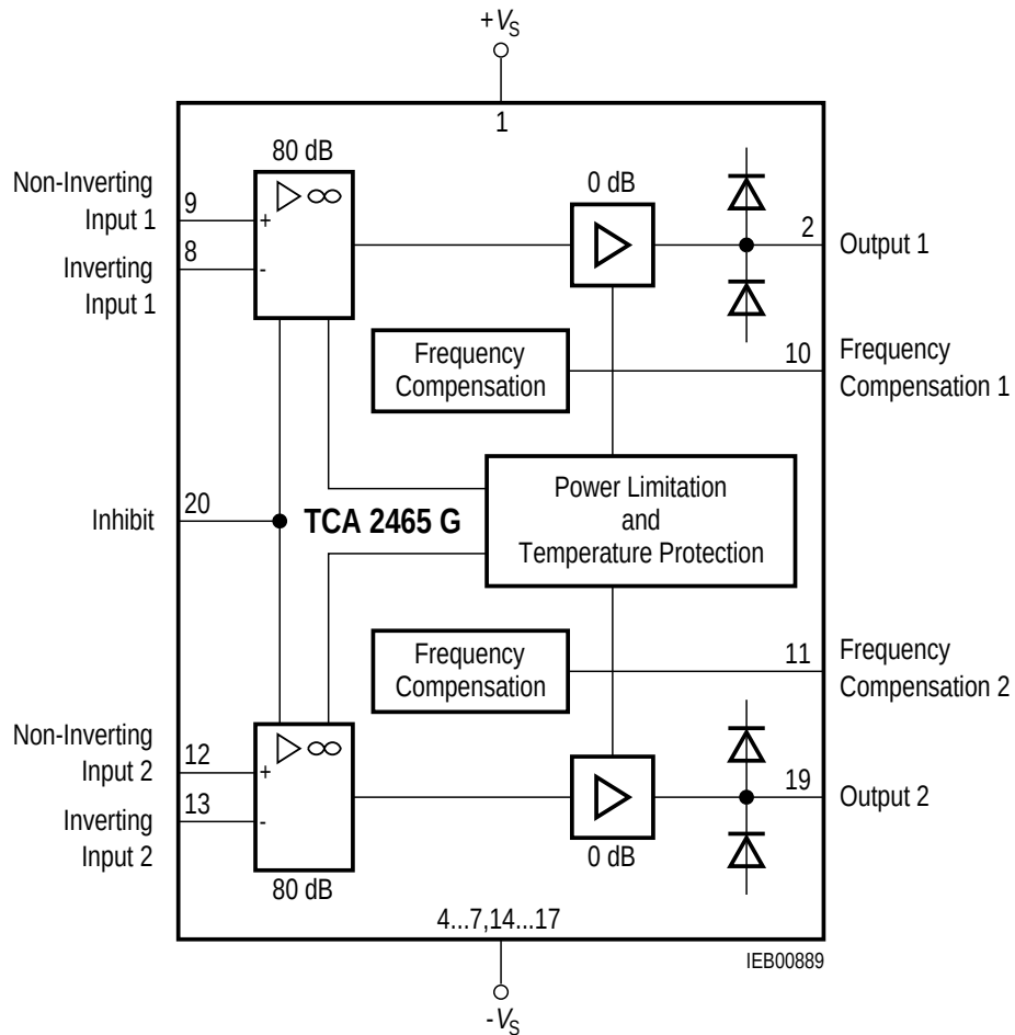
Figure 3 Block Diagram TCA 2465 G
