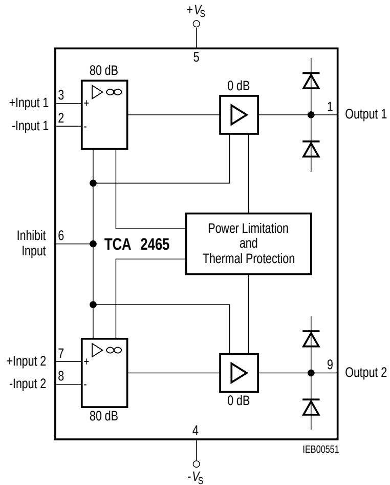
Figure 2 Block Diagram TCA 2465
