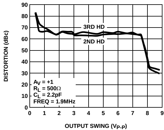
FIGURE 25. DISTORTION vs OUTPUT AMPLITUDE
