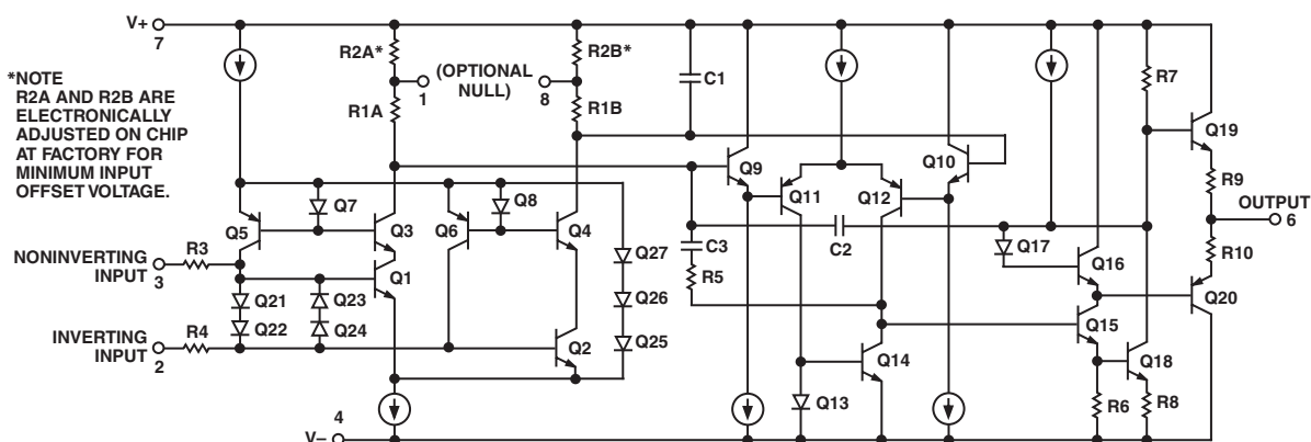
Figure 1. Simplified Schematic
