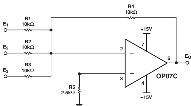
Figure 3. Typical Low Frequency Noise Circuit
