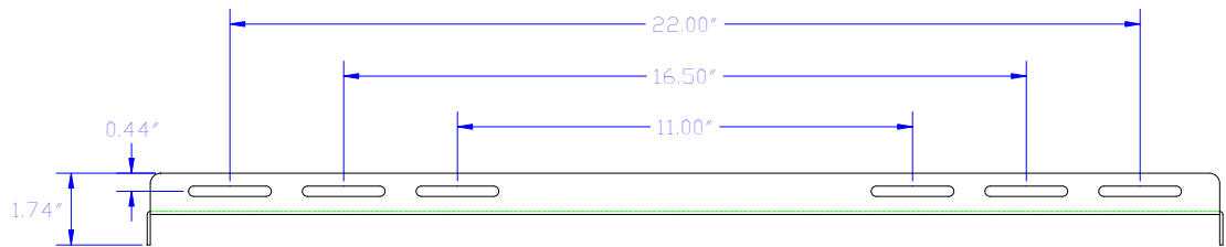
SIDE VIEW
