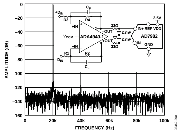
Figure 2. ADA4940-1 Driving the AD7982 ADC
