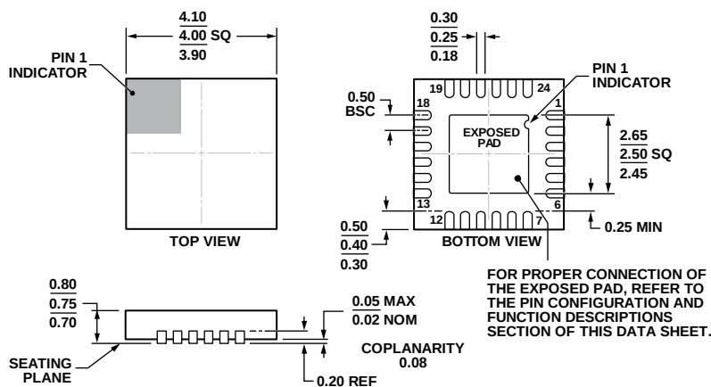
Figure 79. 24-Lead Lead Frame Chip Scale Package [LFCSP_WQ] 4 mm × 4 mm Body, Very Very Thin Quad (CP-24-7)
