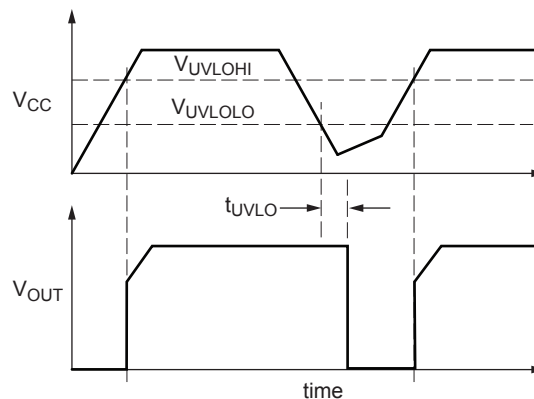
Figure 3. UVLO Operation
