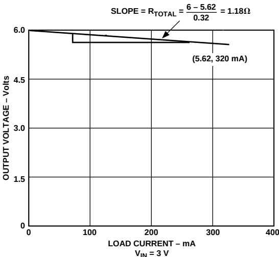
Figure 21. Load Regulation
