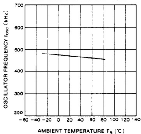
OSCILLATOR FREQUENCY VS. AMBIENT TEMPERATURE (R_{ON}=24k\Omega, R_{OFF}=20k\Omega, C_F=47pF)
