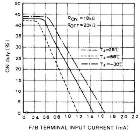
ON duty VS. F/B TERMINAL INPUT CURRENT ( f_{osc}=100\text{kHz} )
