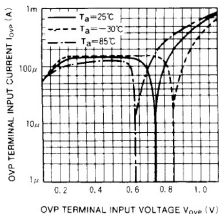
OVP TERMINAL INPUT VOLTAGE VS. INPUT CURRENT
