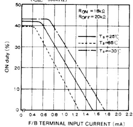
ON duty VS. F/B TERMINAL INPUT CURRENT ( f_{osc}=500\text{kHz} )
