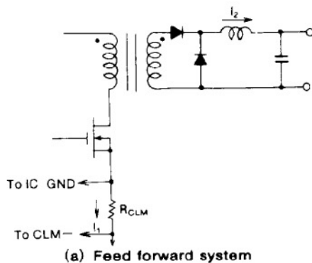
(a) Feed forward system
