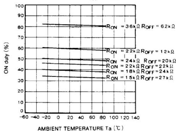
ON duty VS. AMBIENT TEMPERATURE (f_{osc}=100kHz)
