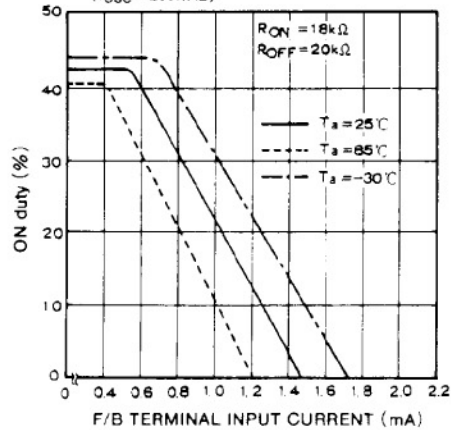
ON duty VS. F/B TERMINAL INPUT CURRENT ( f_{osc}=200\text{kHz} )
