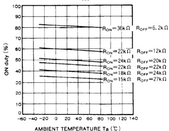
ON duty VS. AMBIENT TEMPERATURE (f_{osc}=500kHz)
