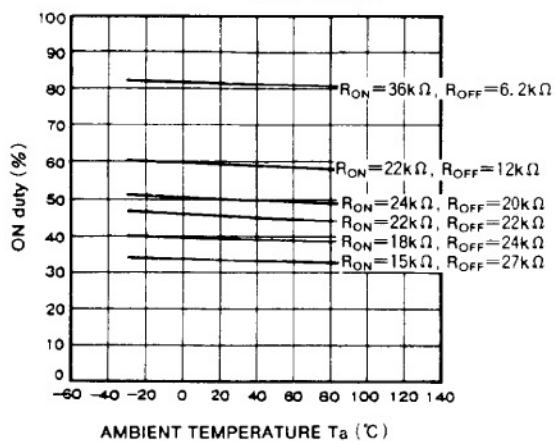
ON duty VS. AMBIENT TEMPERATURE (f_{osc}=200kHz)
