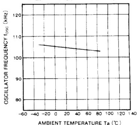
OSCILLATOR FREQUENCY VS. AMBIENT TEMPERATURE (R_{ON}=24k\Omega, R_{OFF}=20k\Omega, C_F=330pF)
