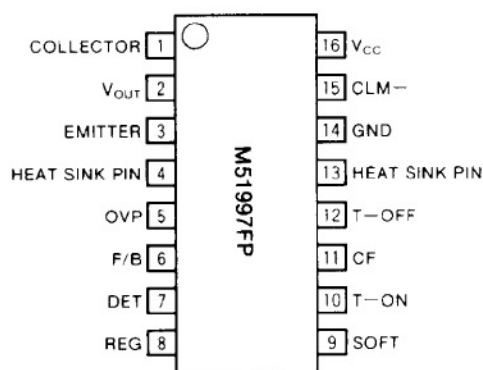
Outline 16P2N-A
