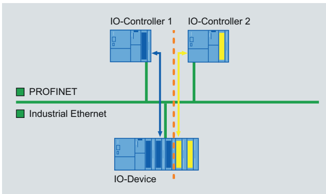
With the Shared Device function, two different IO controllers can access the same IO device simultaneously
