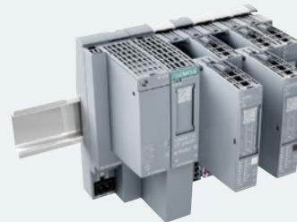
Hot swapping: Module replacement during operation
