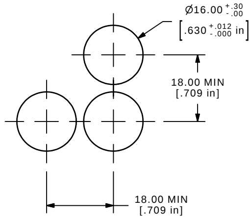
PANEL MOUNTING
